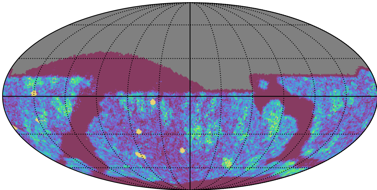
scp_reweight_v3.3_10yrs Yr 1 z band: NVisits
