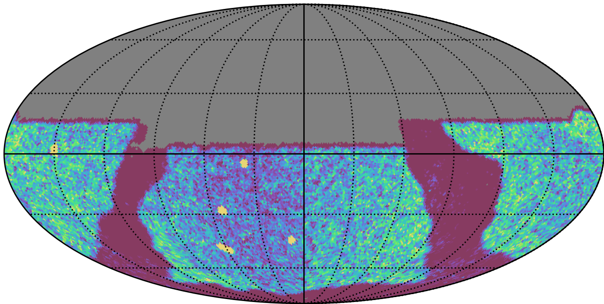
scp_reweight_v3.3_10yrs Yr 1 y band: NVisits
