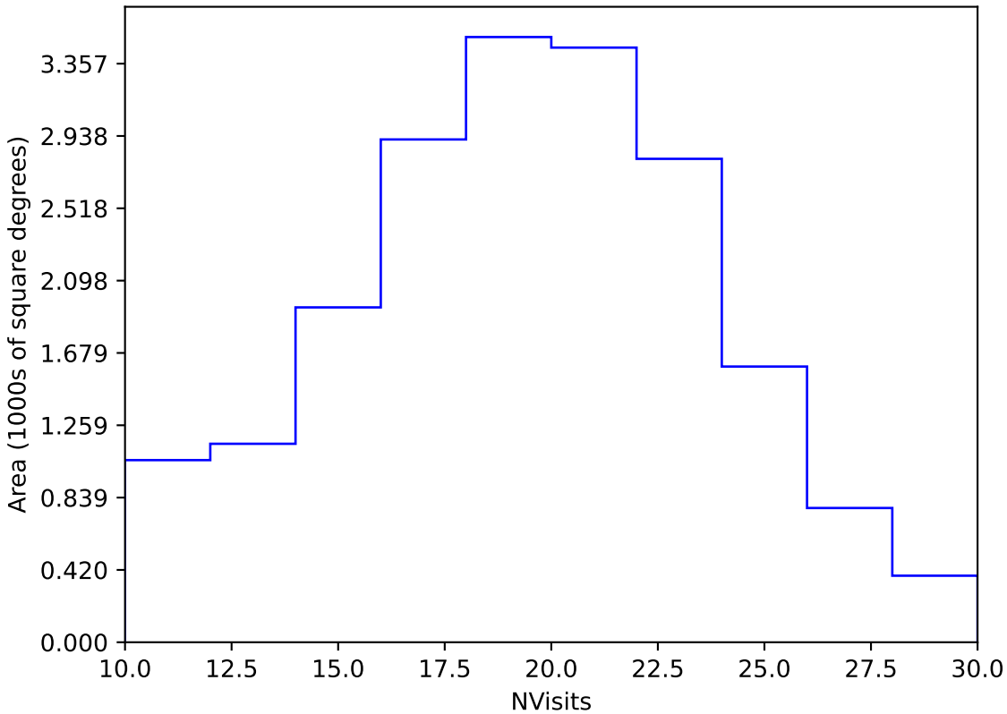
scp_reweight_v3.3_10yrs Yr 1 y band: NVisits
