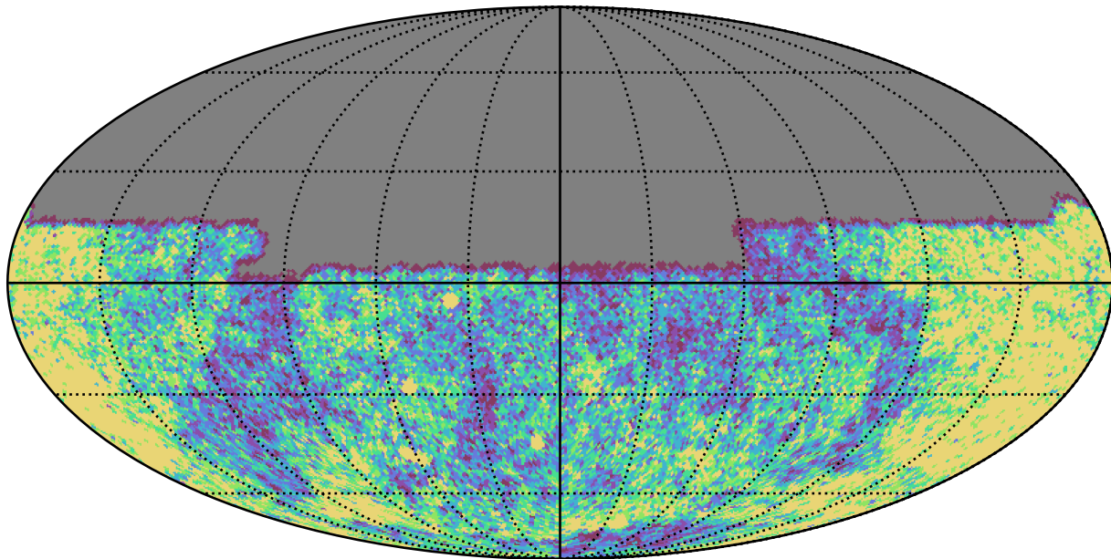
scp_reweight_v3.3_10yrs Yr 1 u band: NVisits
