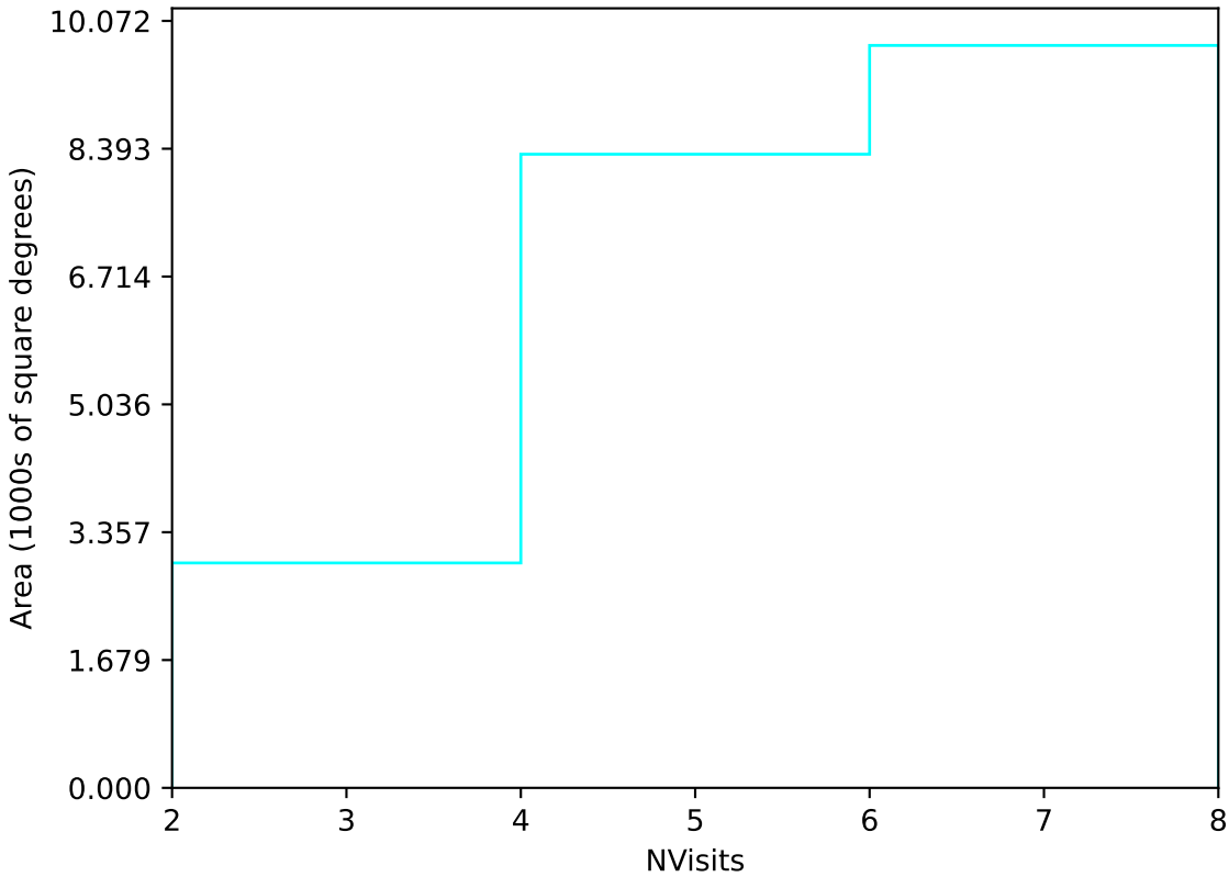
scp_reweight_v3.3_10yrs Yr 1 u band: NVisits
