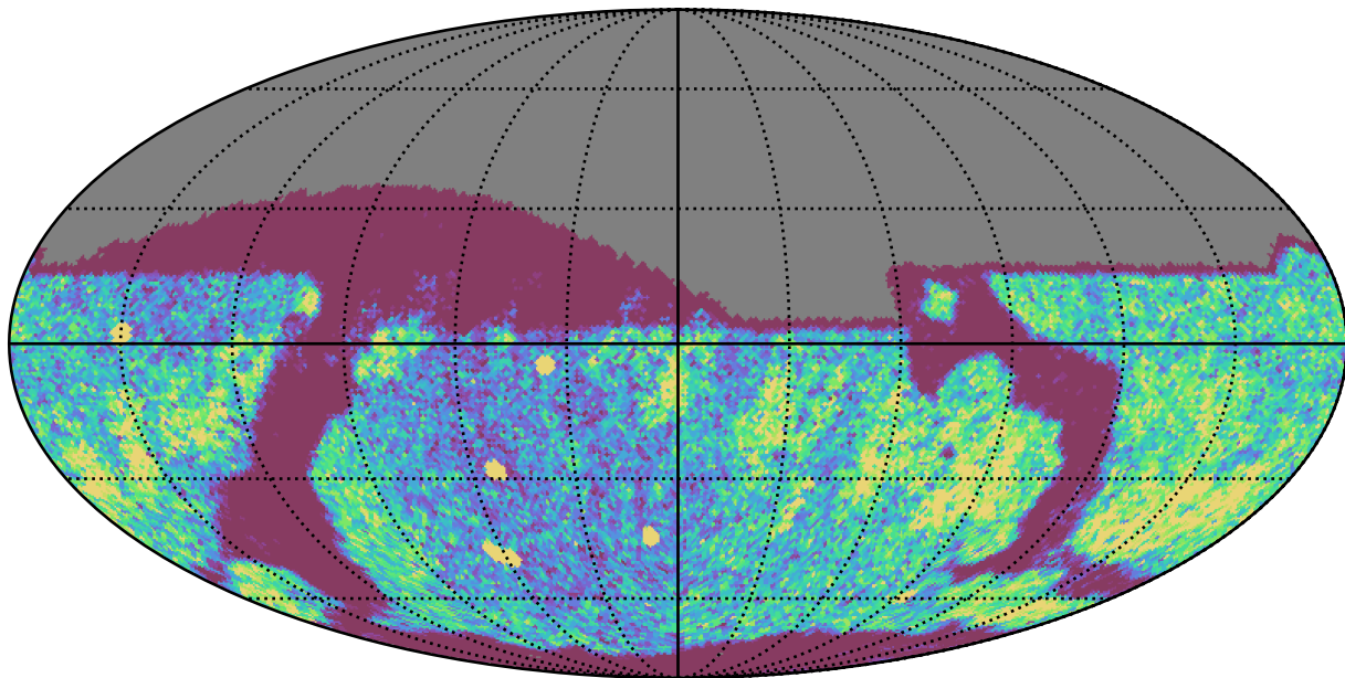
scp_reweight_v3.3_10yrs Yr 1 r band: NVisits
