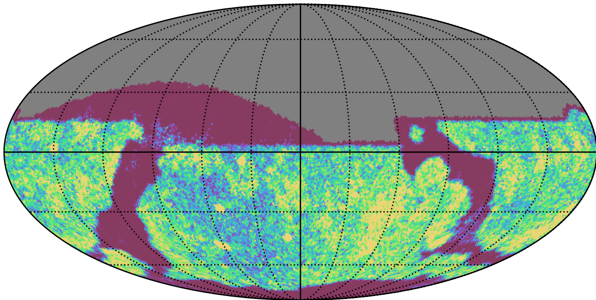
scp_reweight_v3.3_10yrs Yr 1 i band: NVisits
