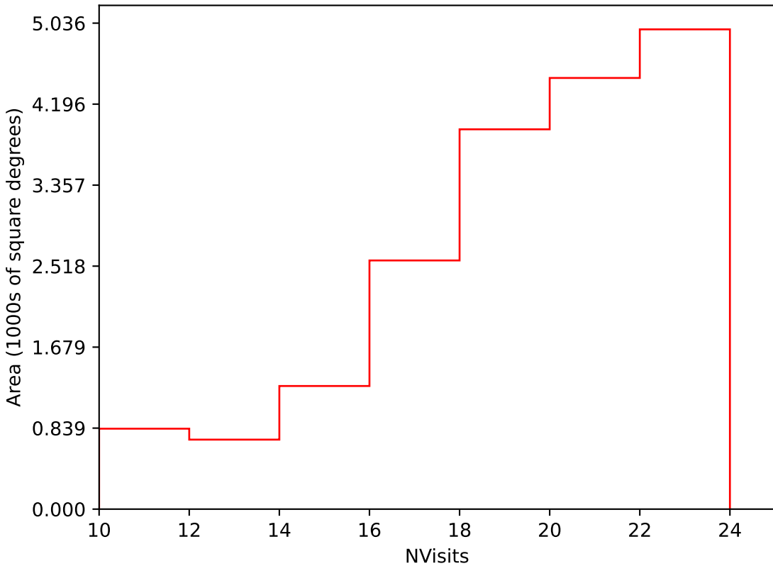
scp_reweight_v3.3_10yrs Yr 1 i band: NVisits
