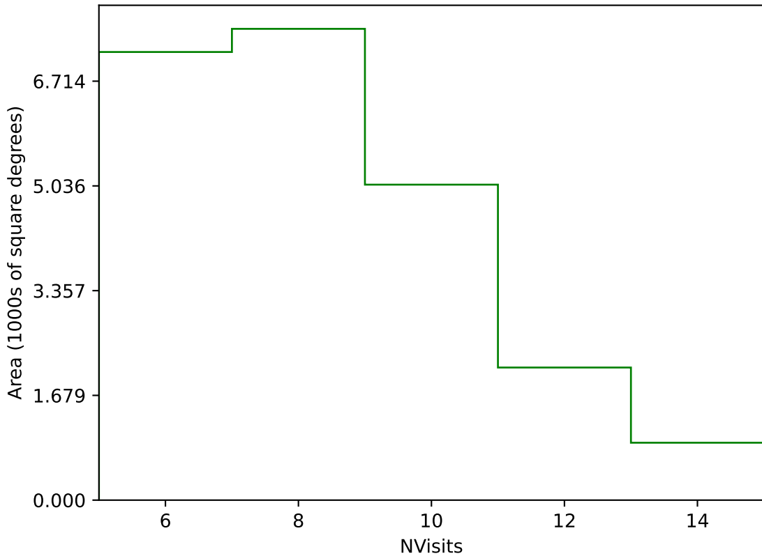
scp_reweight_v3.3_10yrs Yr 1 g band: NVisits
