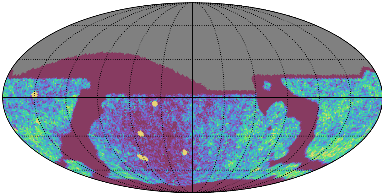
scp_reweight_v3.3_10yrs Yr 1 all bands: NVisits
