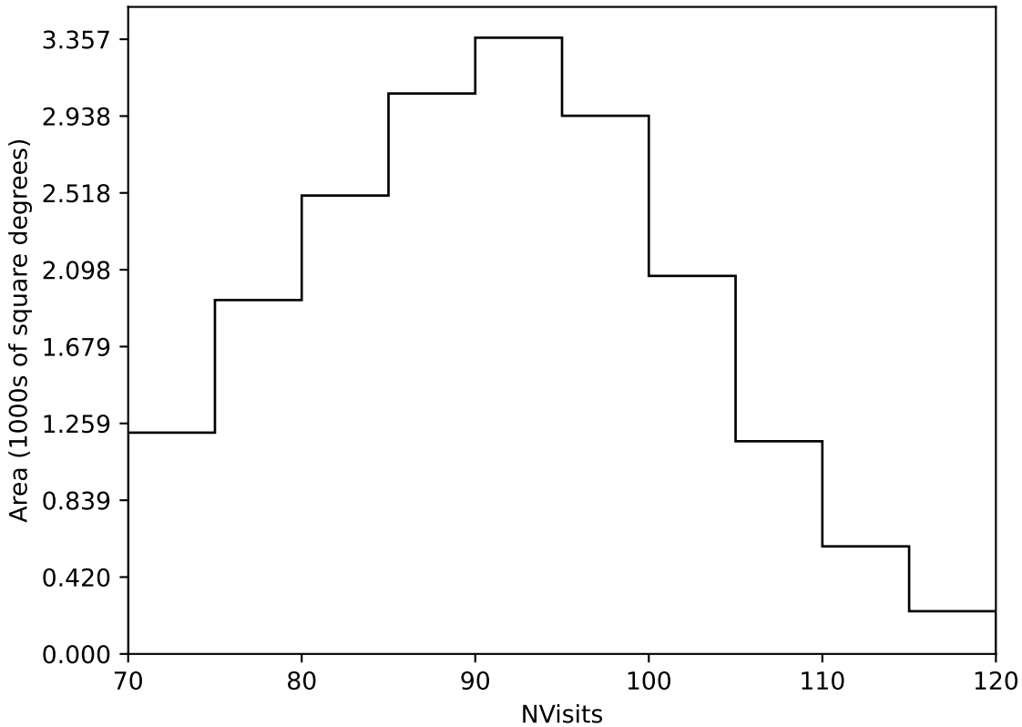
scp_reweight_v3.3_10yrs Yr 1 all bands: NVisits
