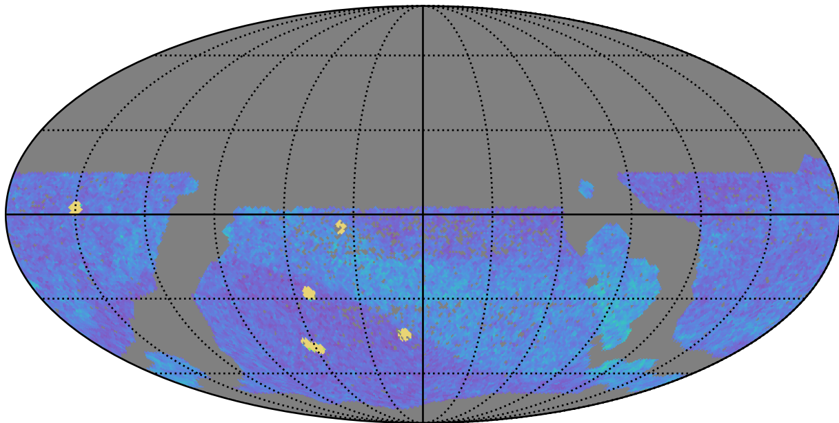
scp_reweight_v3.3_10yrs WFD z band: NVisits
