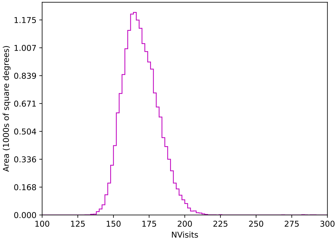
scp_reweight_v3.3_10yrs WFD z band: NVisits
