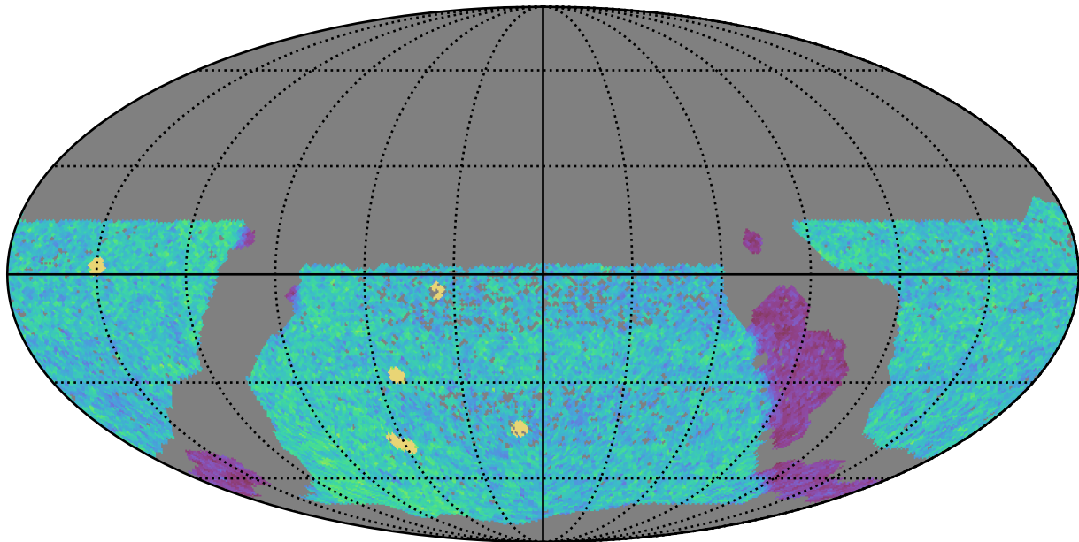
scp_reweight_v3.3_10yrs WFD u band: NVisits
