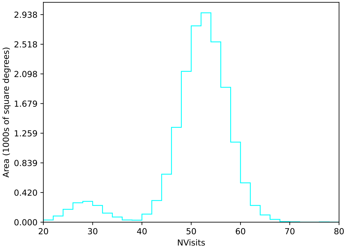
scp_reweight_v3.3_10yrs WFD u band: NVisits
