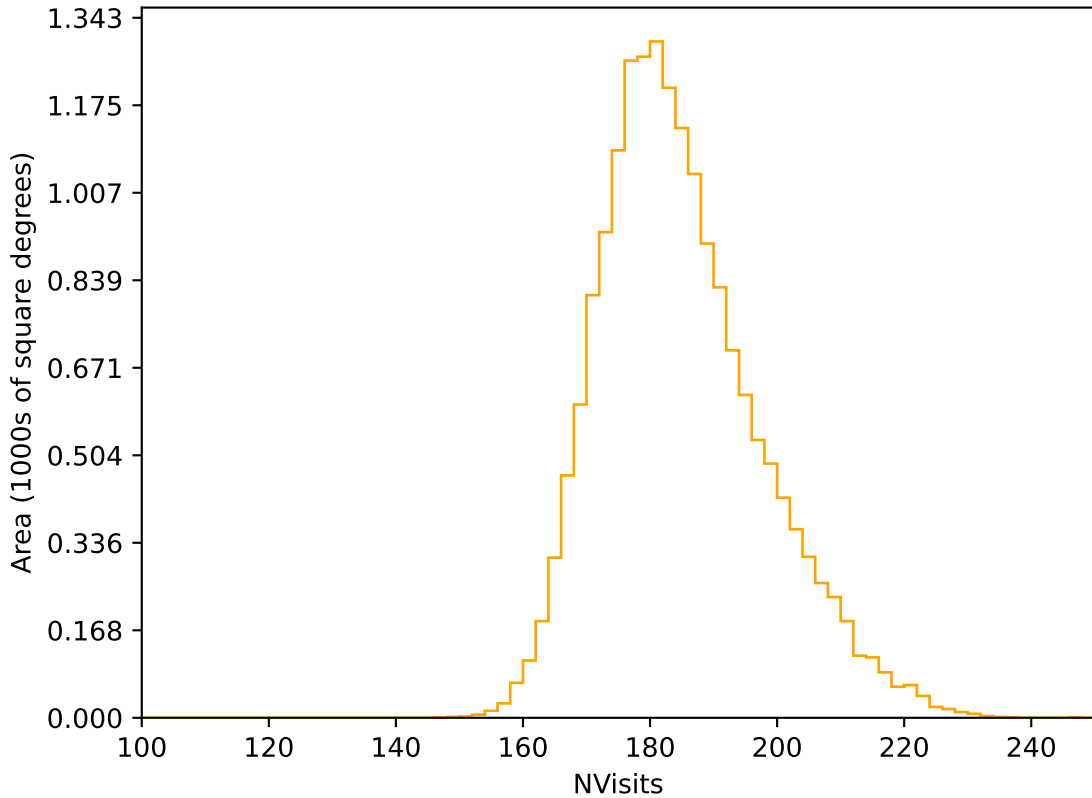
scp_reweight_v3.3_10yrs WFD r band: NVisits
