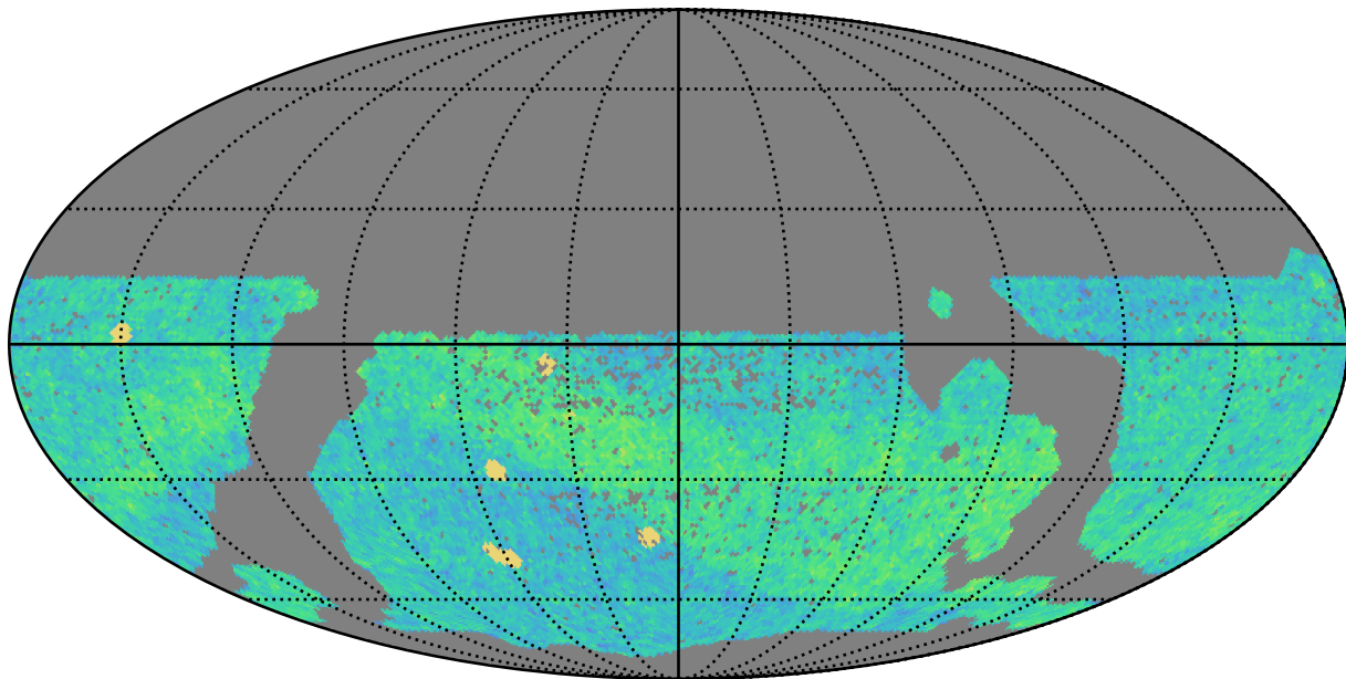
scp_reweight_v3.3_10yrs WFD i band: NVisits
