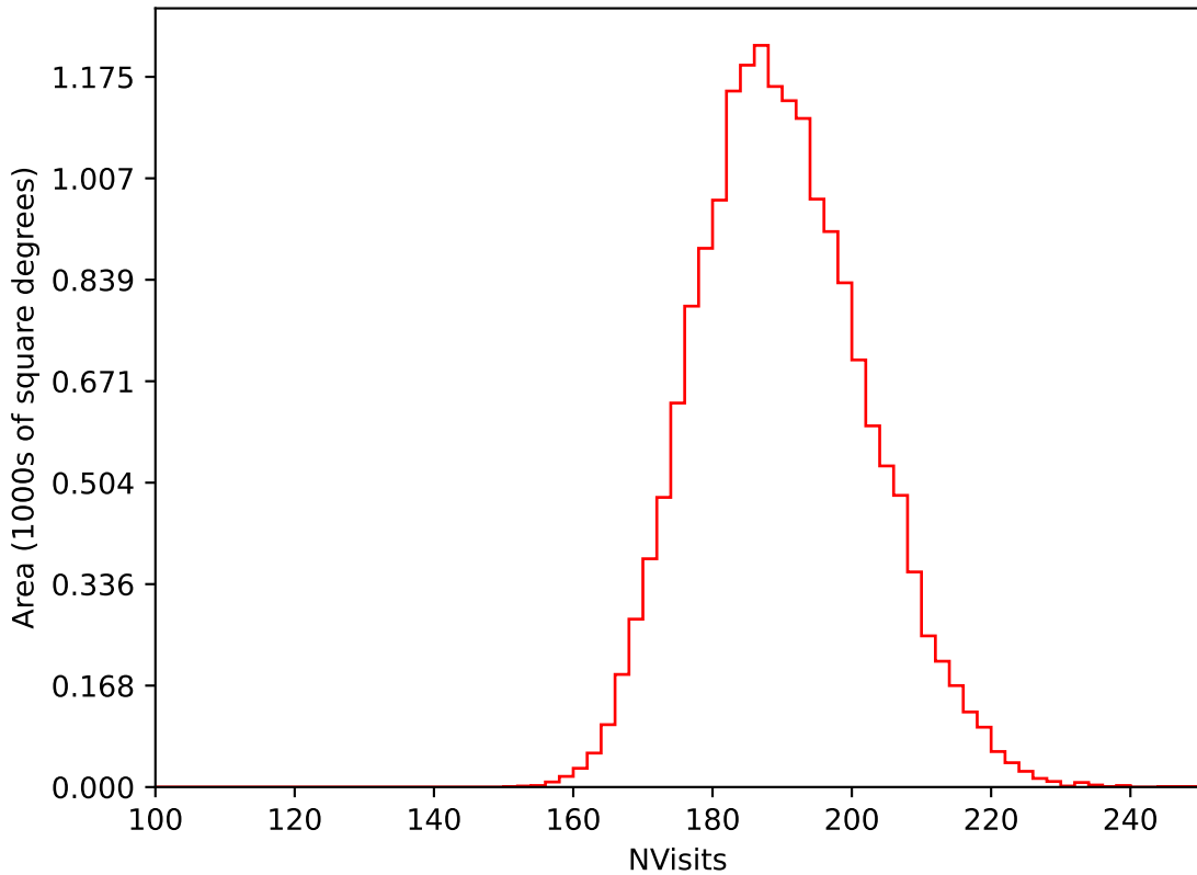
scp_reweight_v3.3_10yrs WFD i band: NVisits
