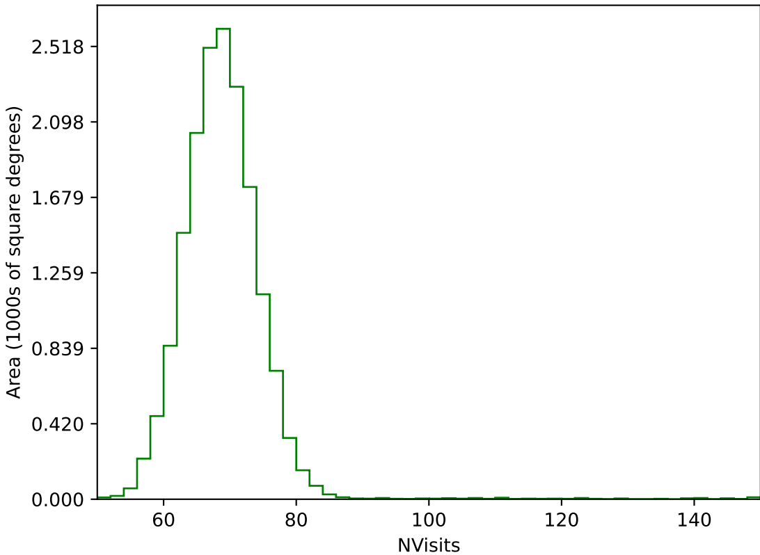
scp_reweight_v3.3_10yrs WFD g band: NVisits
