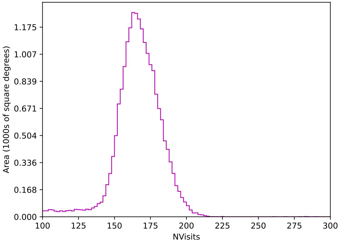
scp_reweight_v3.3_10yrs All sky z band: NVisits
