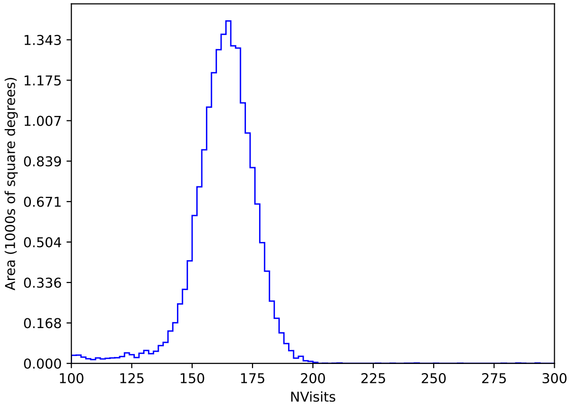
scp_reweight_v3.3_10yrs All sky y band: NVisits
