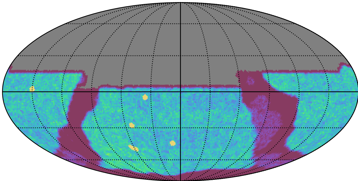
scp_reweight_v3.3_10yrs All sky u band: NVisits
