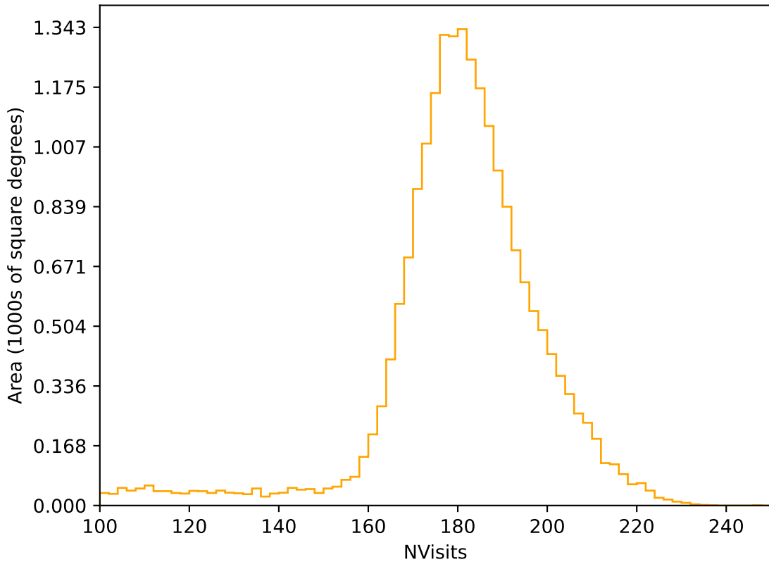
scp_reweight_v3.3_10yrs All sky r band: NVisits
