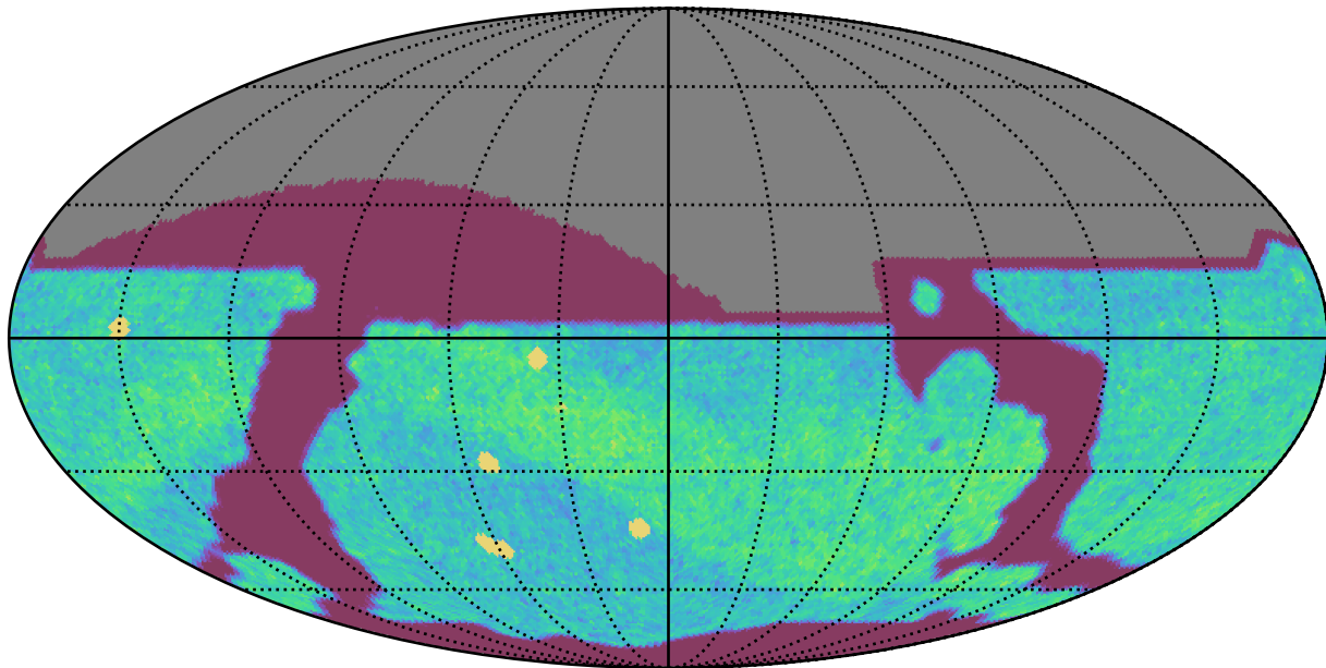
scp_reweight_v3.3_10yrs All sky i band: NVisits
