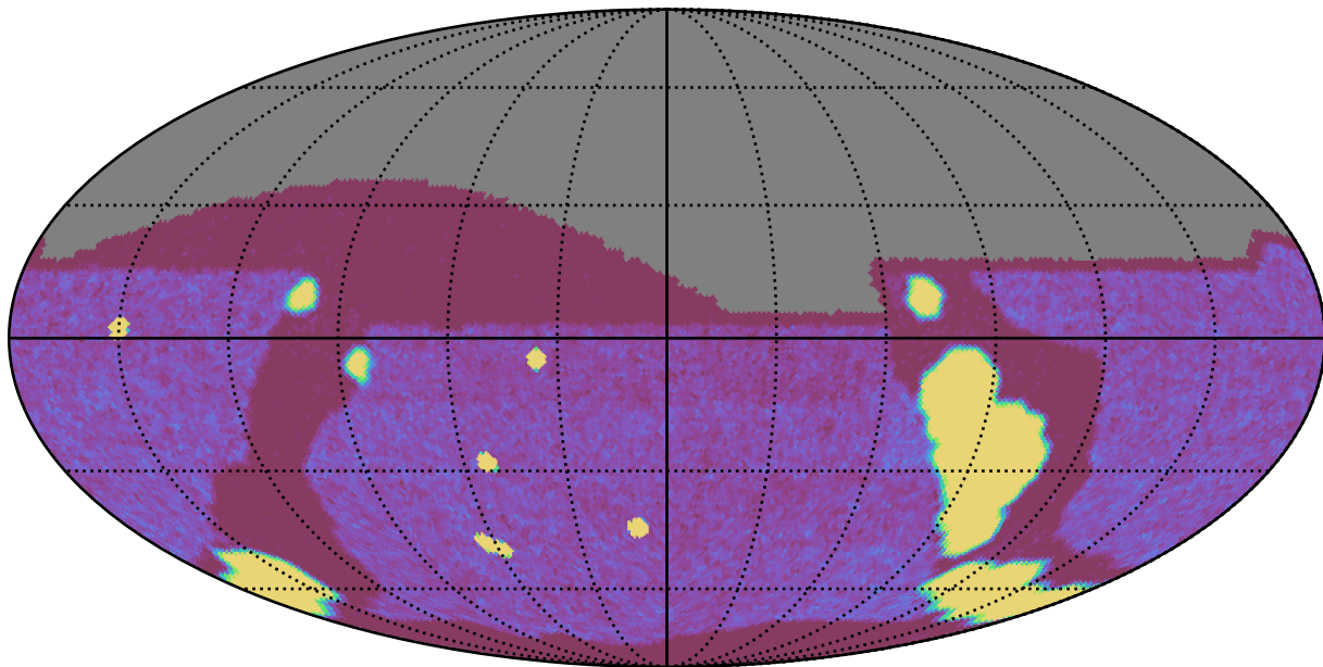
scp_reweight_v3.3_10yrs All sky g band: NVisits
