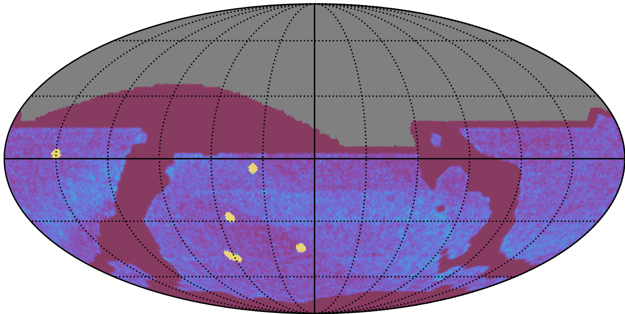
scp_reweight_v3.3_10yrs All sky all bands: NVisits
