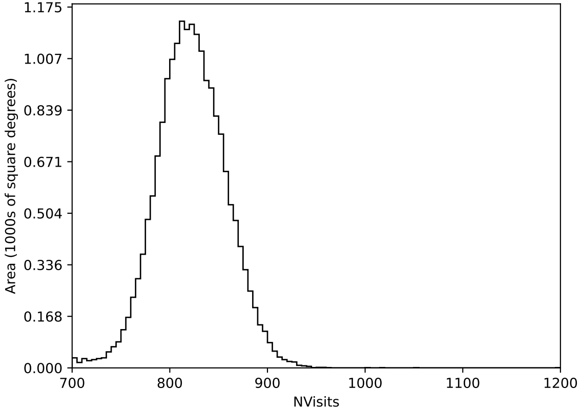
scp_reweight_v3.3_10yrs All sky all bands: NVisits
