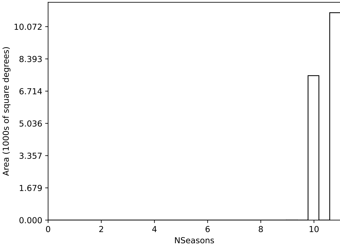
scp_reweight_v3.3_10yrs WFD all bands: NSeasons
