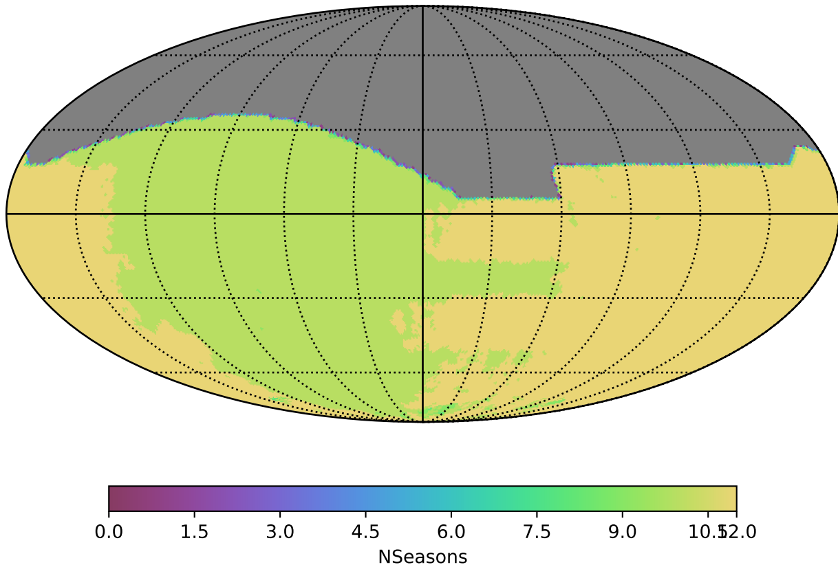
scp_reweight_v3.3_10yrs All sky all bands: NSeasons
