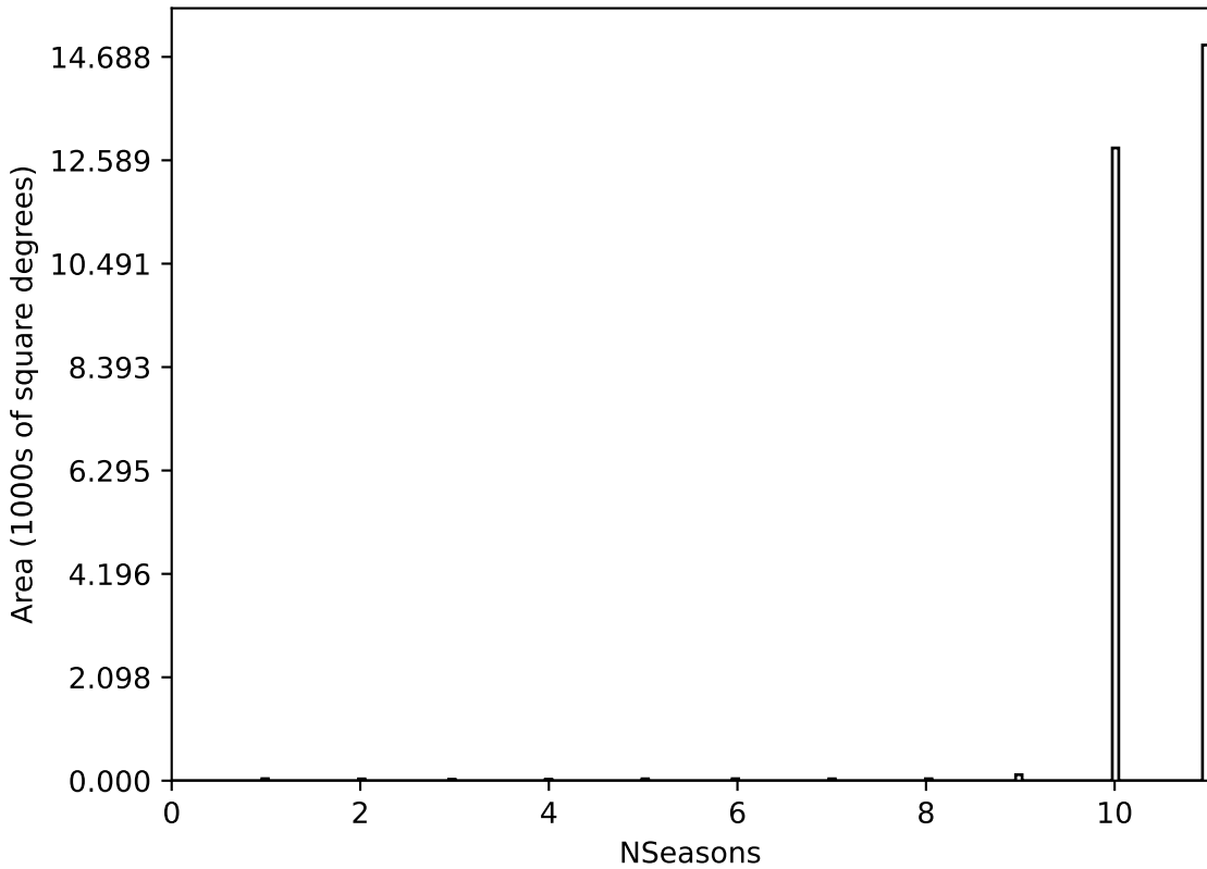
scp_reweight_v3.3_10yrs All sky all bands: NSeasons
