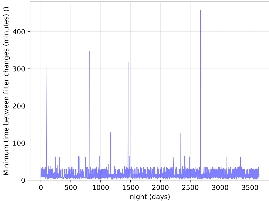
scp_reweight_v3.3_10yrs Per Night: Minimum time between filter changes (minutes)
