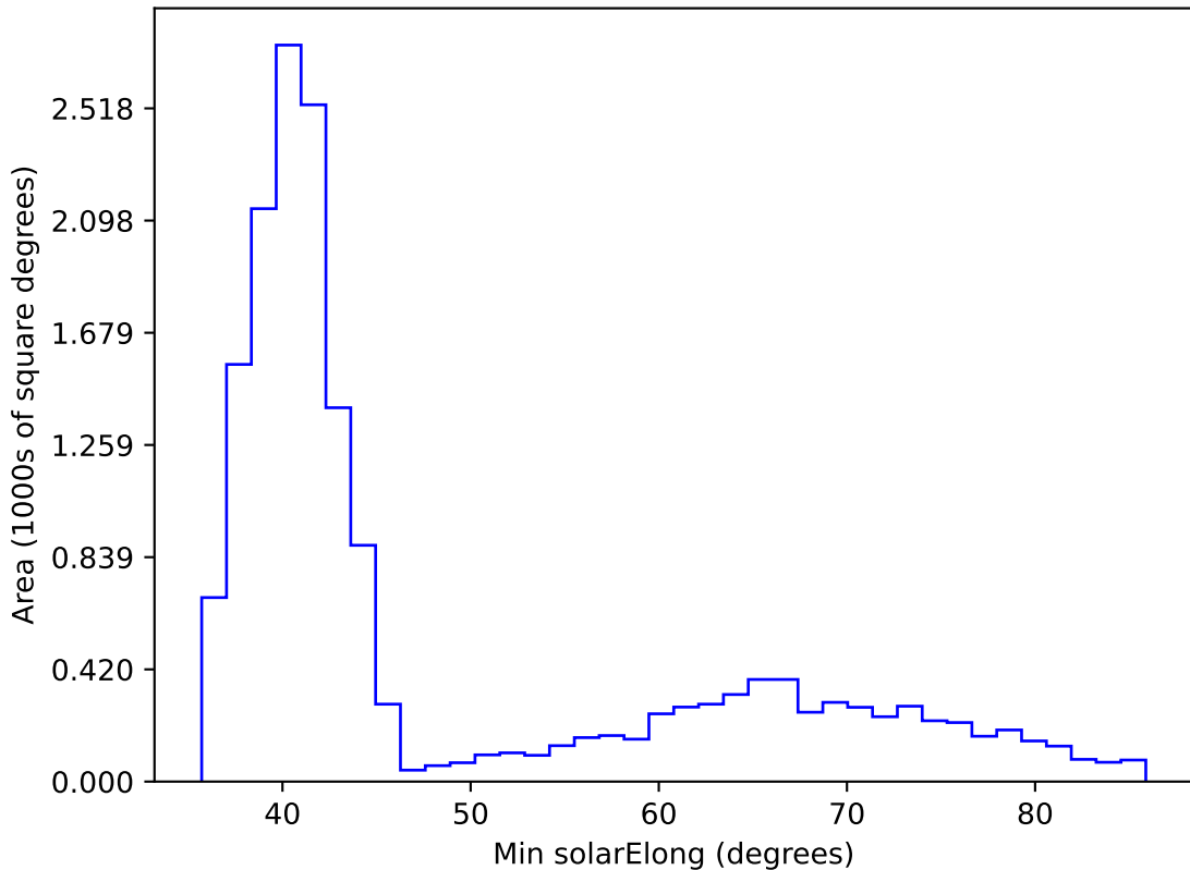
scp_reweight_v3.3_10yrs WFD z band: Min solarElong
