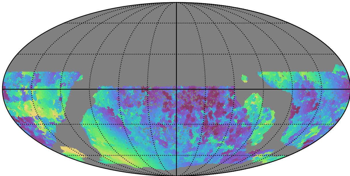
scp_reweight_v3.3_10yrs WFD y band: Min solarElong
