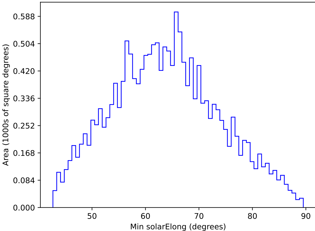
scp_reweight_v3.3_10yrs WFD y band: Min solarElong
