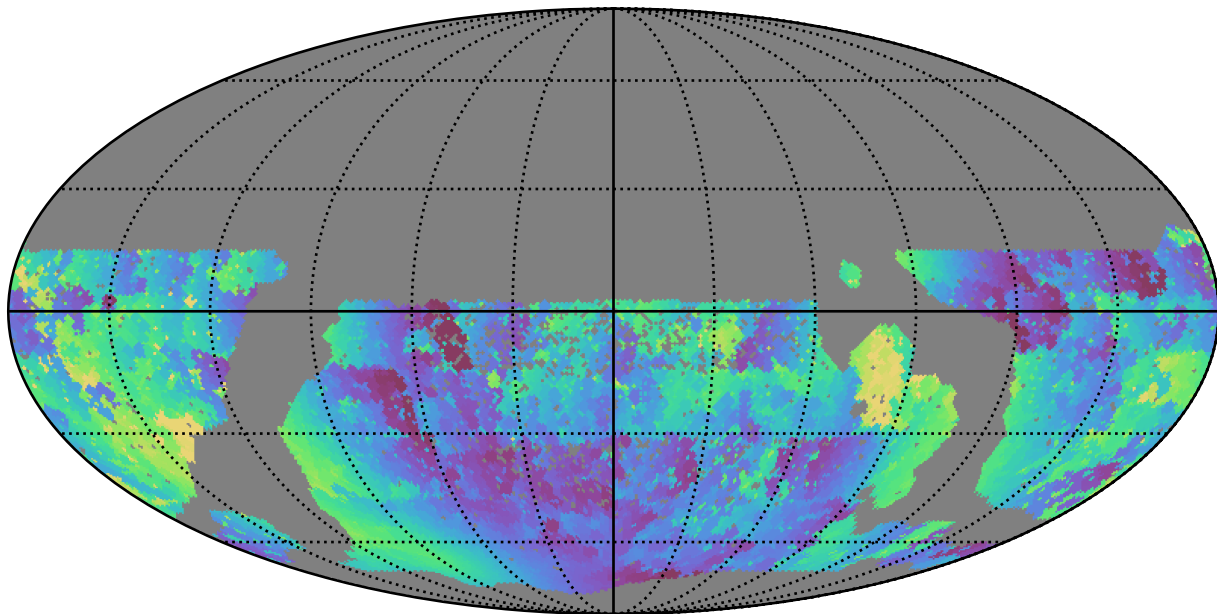
scp_reweight_v3.3_10yrs WFD u band: Min solarElong
