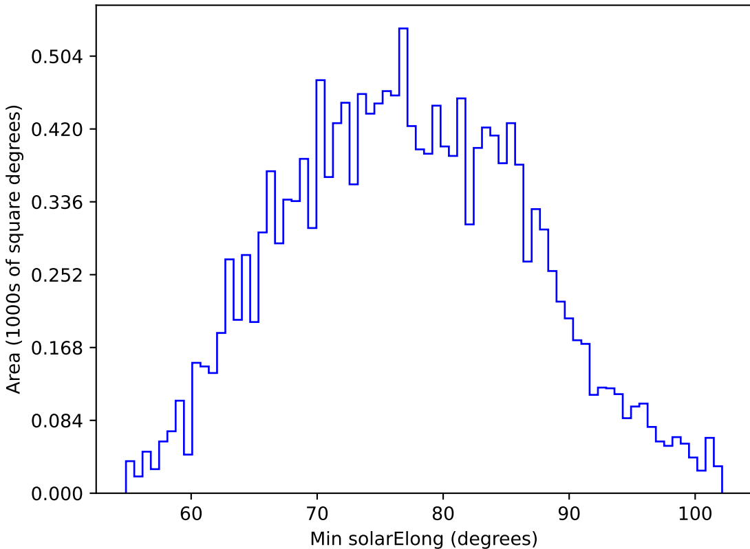
scp_reweight_v3.3_10yrs WFD u band: Min solarElong
