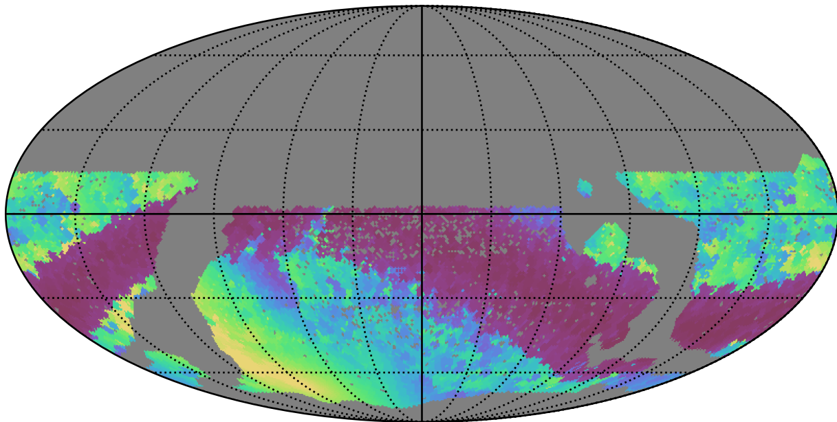
scp_reweight_v3.3_10yrs WFD r band: Min solarElong
