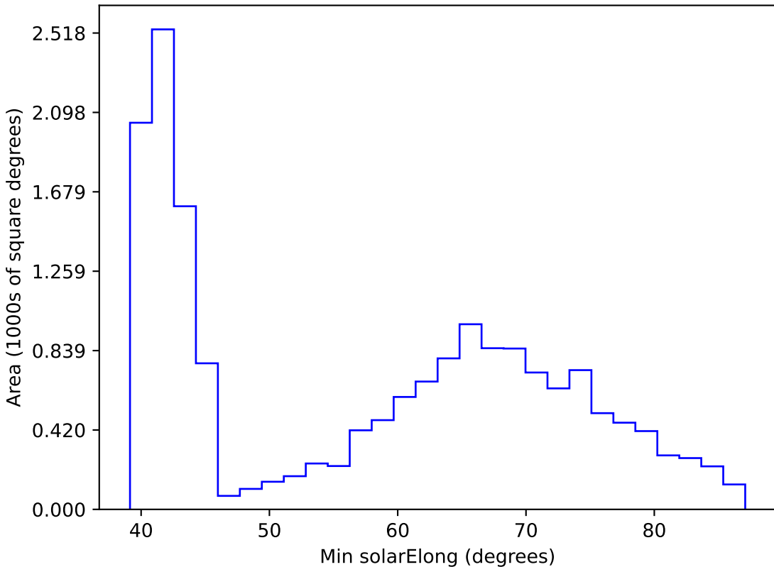
scp_reweight_v3.3_10yrs WFD r band: Min solarElong
