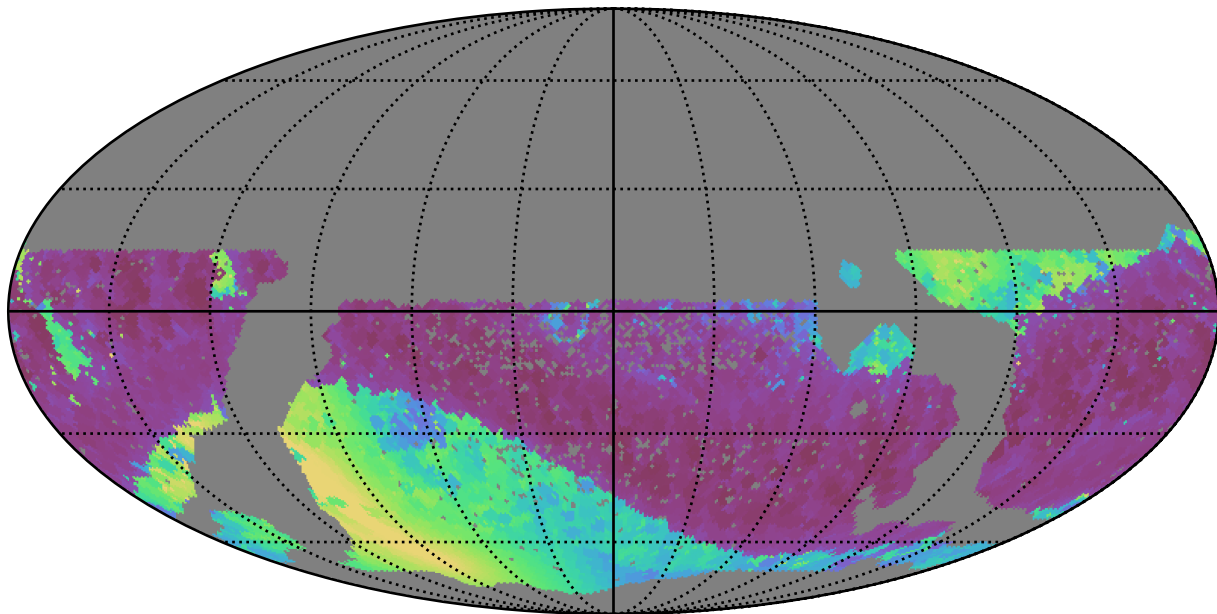
scp_reweight_v3.3_10yrs WFD i band: Min solarElong
