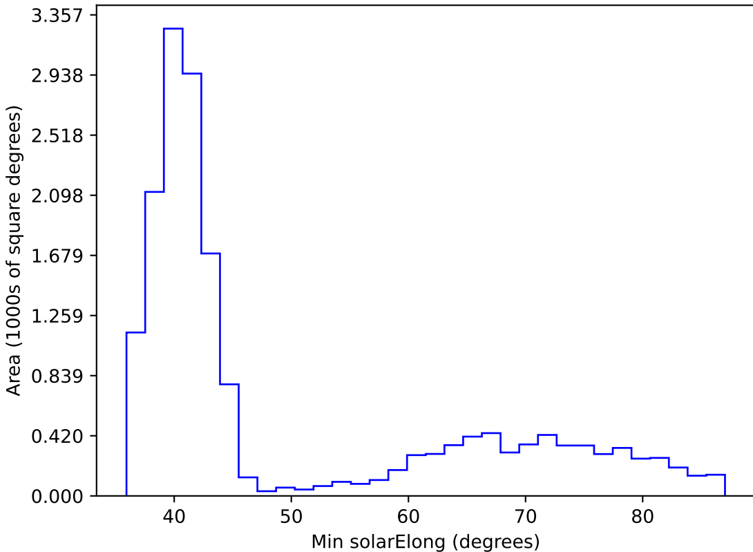
scp_reweight_v3.3_10yrs WFD i band: Min solarElong
