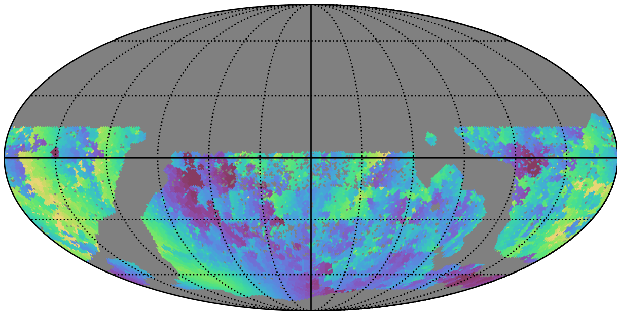
scp_reweight_v3.3_10yrs WFD g band: Min solarElong
