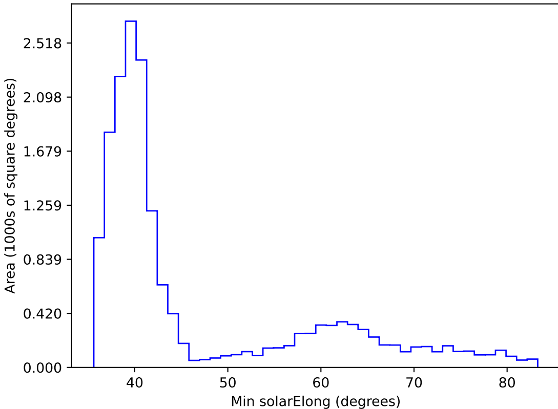
scp_reweight_v3.3_10yrs WFD all bands: Min solarElong
