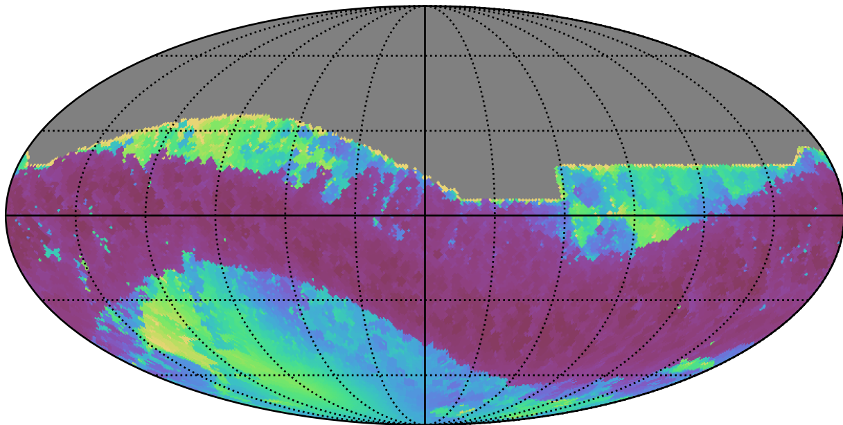
scp_reweight_v3.3_10yrs All sky z band: Min solarElong
