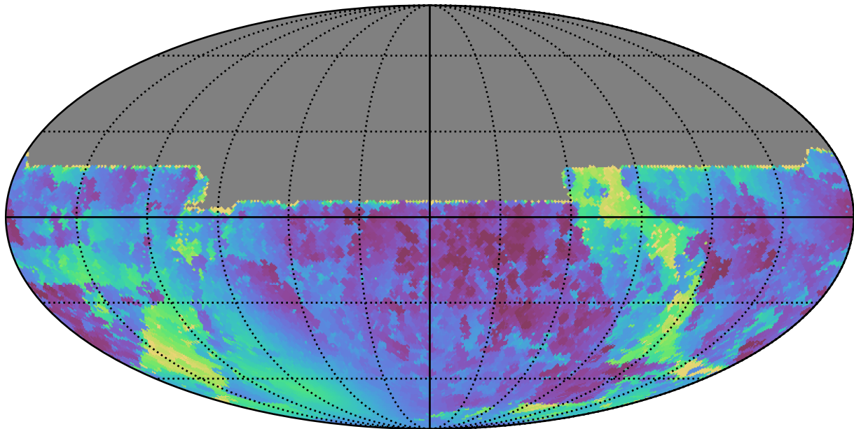
scp_reweight_v3.3_10yrs All sky y band: Min solarElong
