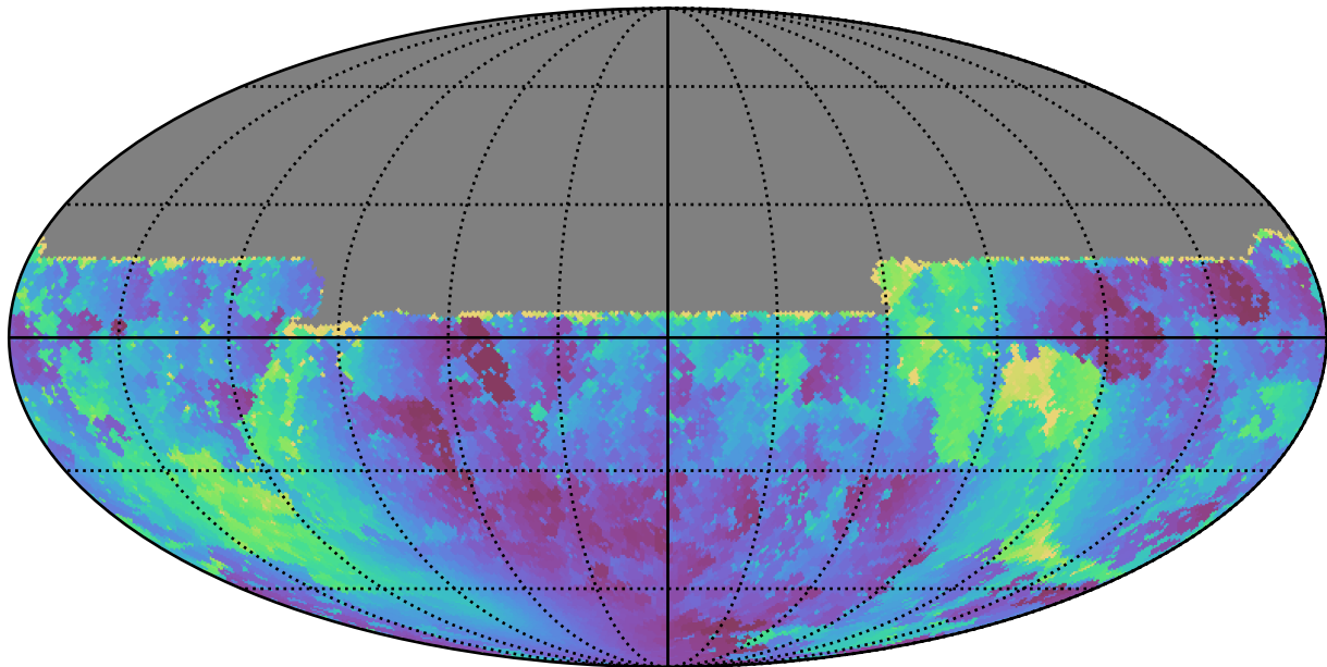
scp_reweight_v3.3_10yrs All sky u band: Min solarElong
