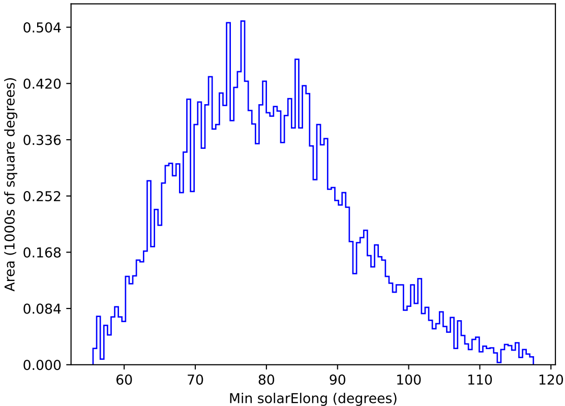
scp_reweight_v3.3_10yrs All sky u band: Min solarElong
