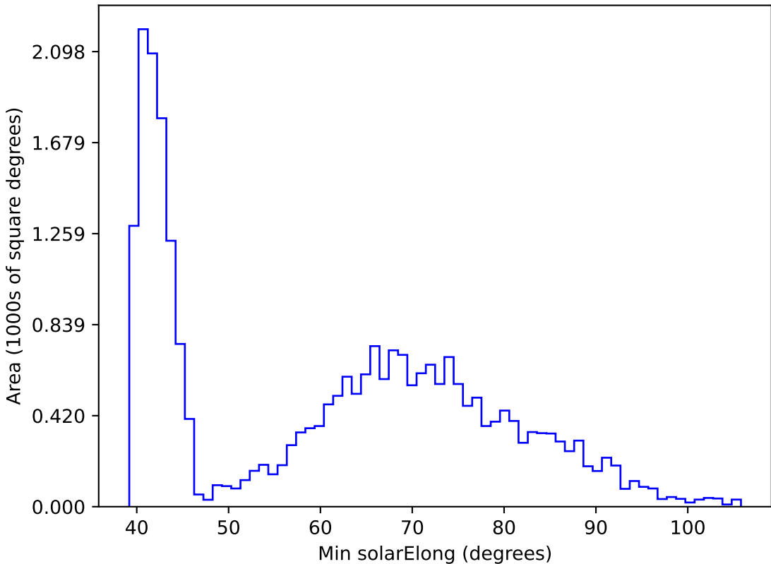
scp_reweight_v3.3_10yrs All sky r band: Min solarElong
