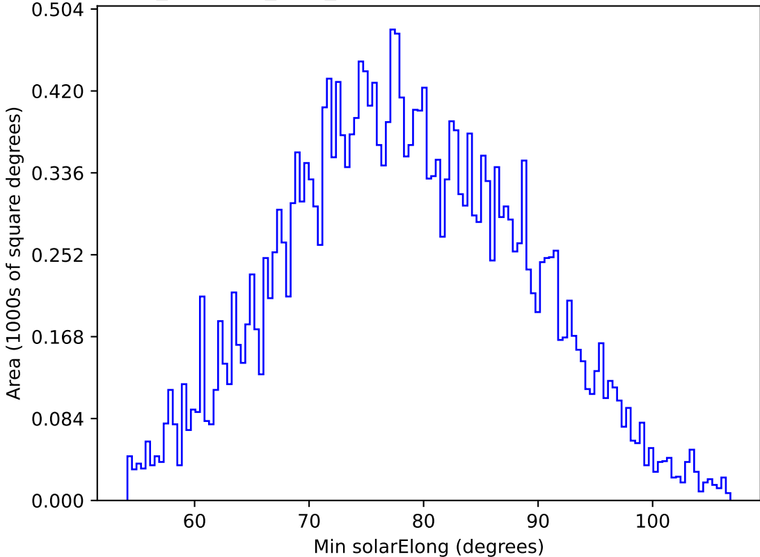
scp_reweight_v3.3_10yrs All sky g band: Min solarElong
