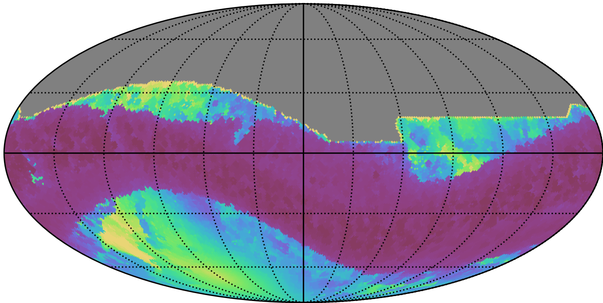
scp_reweight_v3.3_10yrs All sky all bands: Min solarElong
