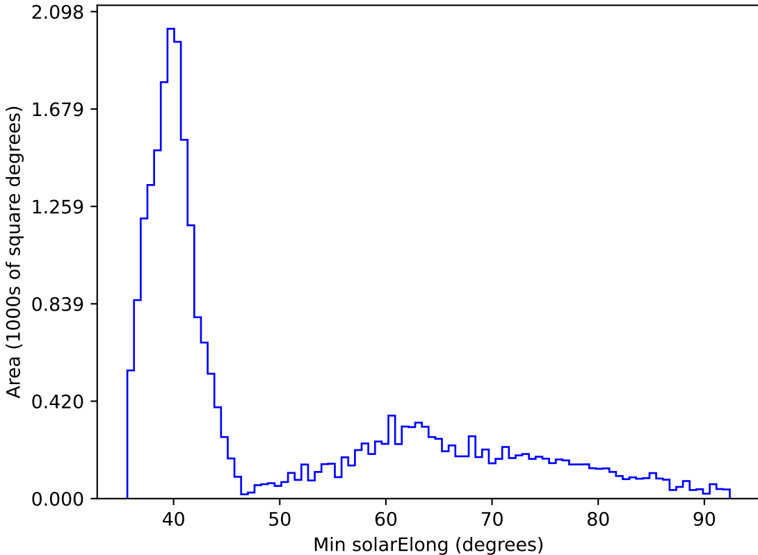
scp_reweight_v3.3_10yrs All sky all bands: Min solarElong
